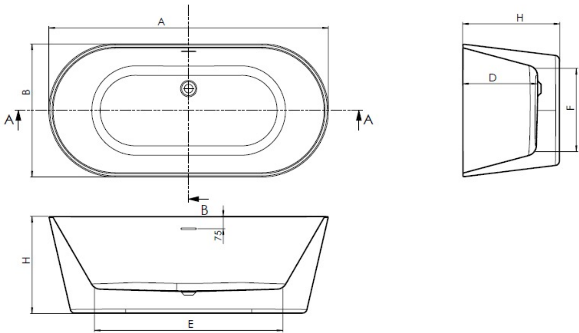
Technical drawing
