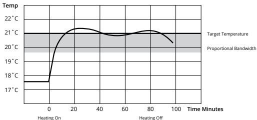
Graph (20.1): TPI Control
